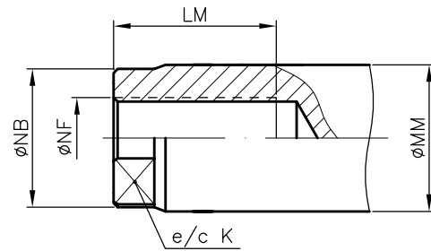
Roscado interior – 2
