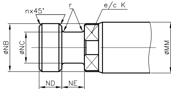
Tenon – 3
